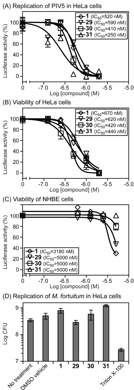
Figure 5. (A–C) Dose-dependent effects of compounds 1 and 29–31 on renilla luciferase expressed by rPIV5-RL in HeLa cells (A), on viability of HeLa cells after 24 h (B), and on viability of NHBE cells after 40 h (C). Viability of mammalian cells was measured by quantification of cellular ATP with firefly luciferase. (D) Examination of effects of compounds (0.5 \mu M) compared with Triton X-100 (1%) on replication of intracellular M. fortuitum bacteria in HeLa cells. Data are in triplicate or larger numbers of measurements. Standard errors of the mean are \leq 20%.
