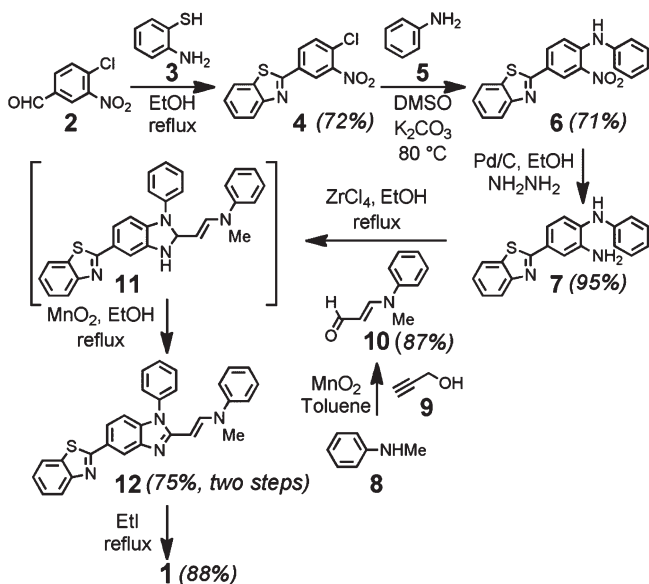
Scheme 1. Synthesis of AKT Inhibitor-IV ( 1 )
