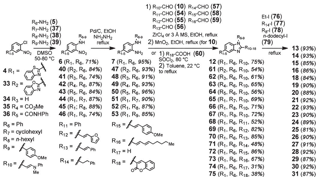
Scheme 2. Synthesis of 13–16 and 18–31
