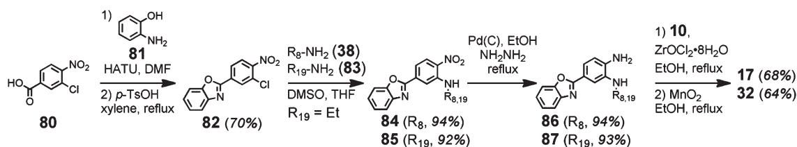
Scheme 3. Synthesis of 17 and 32
