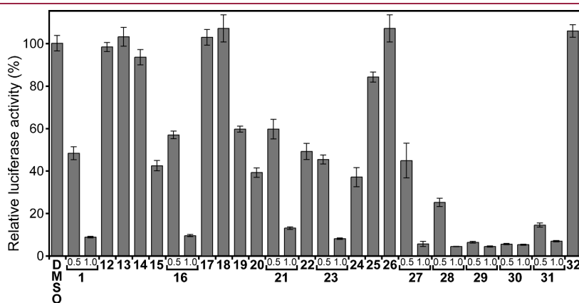
Figure 4. Initial evaluation of compounds 1 and 12 – 32 against rPIV5-RL at one day post infection. All compounds were tested at 1 \mu\text{M} . Compounds comparable in activity to 1 were further examined at 0.5 \mu\text{M} (concentrations ( \mu\text{M} ) shown in brackets). Error bars represent standard errors of the mean.
