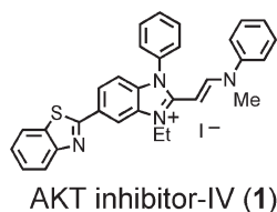
Figure 1. Structure of AKT inhibitor IV (1).
