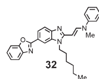
Figure 2. Structures of analogues 12–32. For 13–16 and 18–31, compounds were isolated as ammonium iodides.
